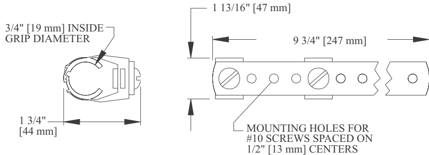
STANDARD MOUNTING BRACKET
